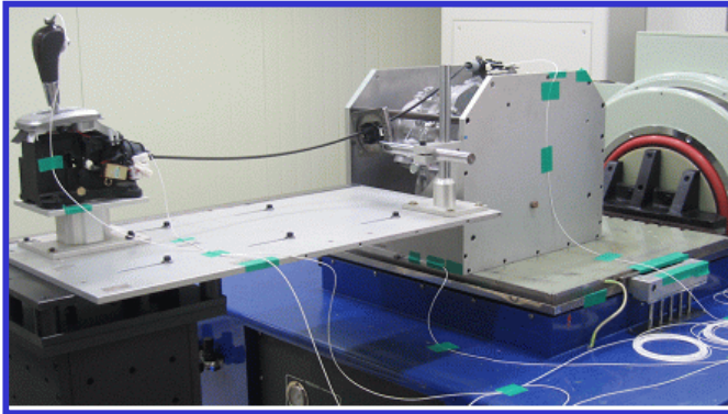
Daedong Systems Co., Ltd. for GM-DAT : Transmission Cable Vibration Test
