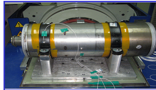
Daeji Metal Co., Ltd. for Doosan Infracore : Muffler Vibration Test
